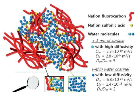
Figure 3. Schematic summary of the distinctly heterogeneous water and proton diffusivity. D_p and D_w are the diffusion constants of proton and water, respectively, as measured by 1 H ODNP relaxometry. The D_p and D_w values were found to vary dramatically across the heterogeneous Nafion membrane structure encompassing water channels, sulfonic acid groups, and a fluorocarbon-based polymer phase, with significantly higher D_p and D_w values found near the fluorocarbon interface of the water channels.
